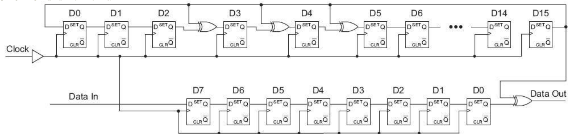
LFSR skrembler
